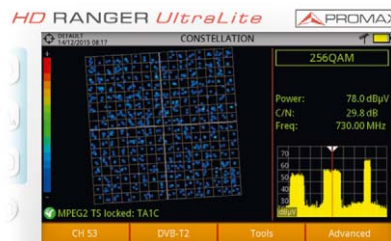
Constellation diagram
