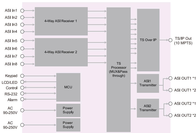
Functional Block Diagram (Multi Channel Mode)
